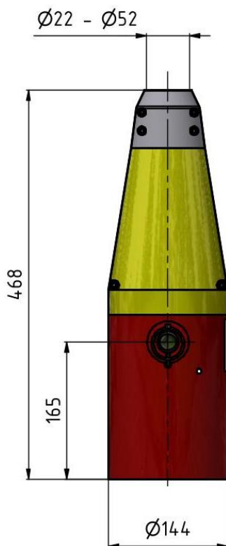
GO.45.100.P1 2 pins
